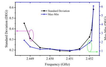
Fig. 2. Standard deviation and maximum peak-to-peak difference values as a function of the frequency of the injected signal. [3]
