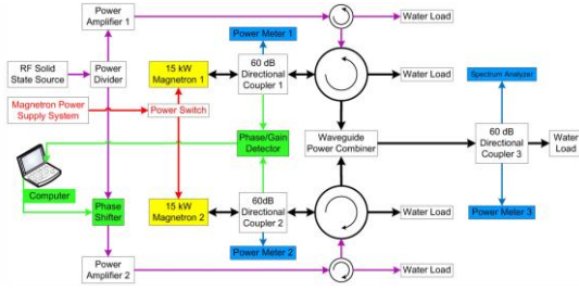
Fig. 4 The block diagram of two-way injection-locked 15 kW CW magnetrons microwave power combining system. [5]
