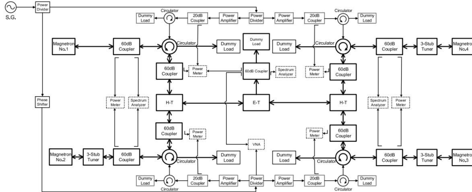
Fig. 6 Diagram of the 60-kW CW magnetron microwave power combining system. Dashed line framework part: measurement setup. Connected to signal generator (top and bottom) injection signal route. Highlighted middle part: high-power output route[7]
