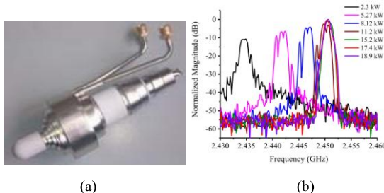
Fig. 1. Magnetron and the output spectrum. (a) Water-cool 20kW CW magnetron. (b) Magnetron output spectrum at various output power.[2]
