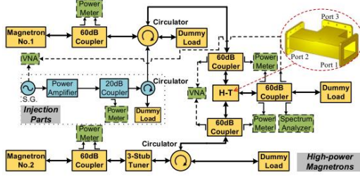
Fig. 5. Diagram of the phase-shifterless magnetron power controlled combining system.[6]
