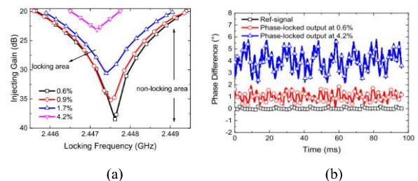
Fig. 3. Measurement results. (a) Phase-locking areas with respect to the anode voltage ripples. (b) Phase jitters with respect to various anode voltage ripples.[4]
